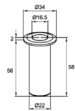
Bolt Keeper
